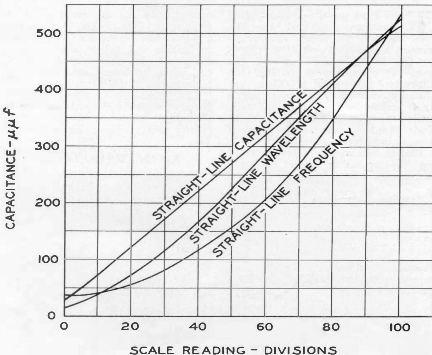
FIGURE 1. Capacitance calibrations for three typical General Radio condensers: (a) Straight-line capacitance, TYPE 247-G; (b) Straight-line wavelength, TYPE 247-F; (c) Straight-line frequency, TYPE 374-F
