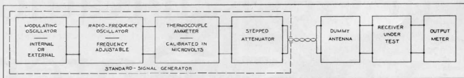
FIGURE 2. Outline showing component parts of the standard-signal generator and auxiliary equipment required for making sensitivity, selectivity, and fidelity characteristics on radio receivers
