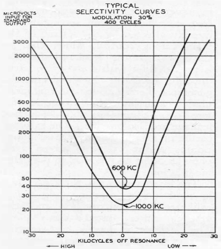
Typical broadcast receiver characteristics: FIGURE 4—Sensitivity curve; FIGURE 5—Selectivity curve; FIGURE 6—Fidelity curve
