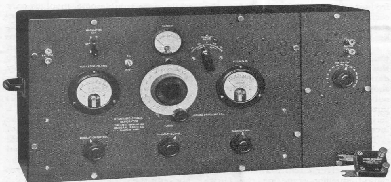
FIGURE 1. TYPE 403-C Standard-Signal Generator, front of panel view
