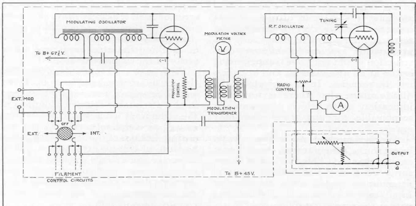
FIGURE 3. Functional schematic of TYPE 403-C Standard-Signal Generator
